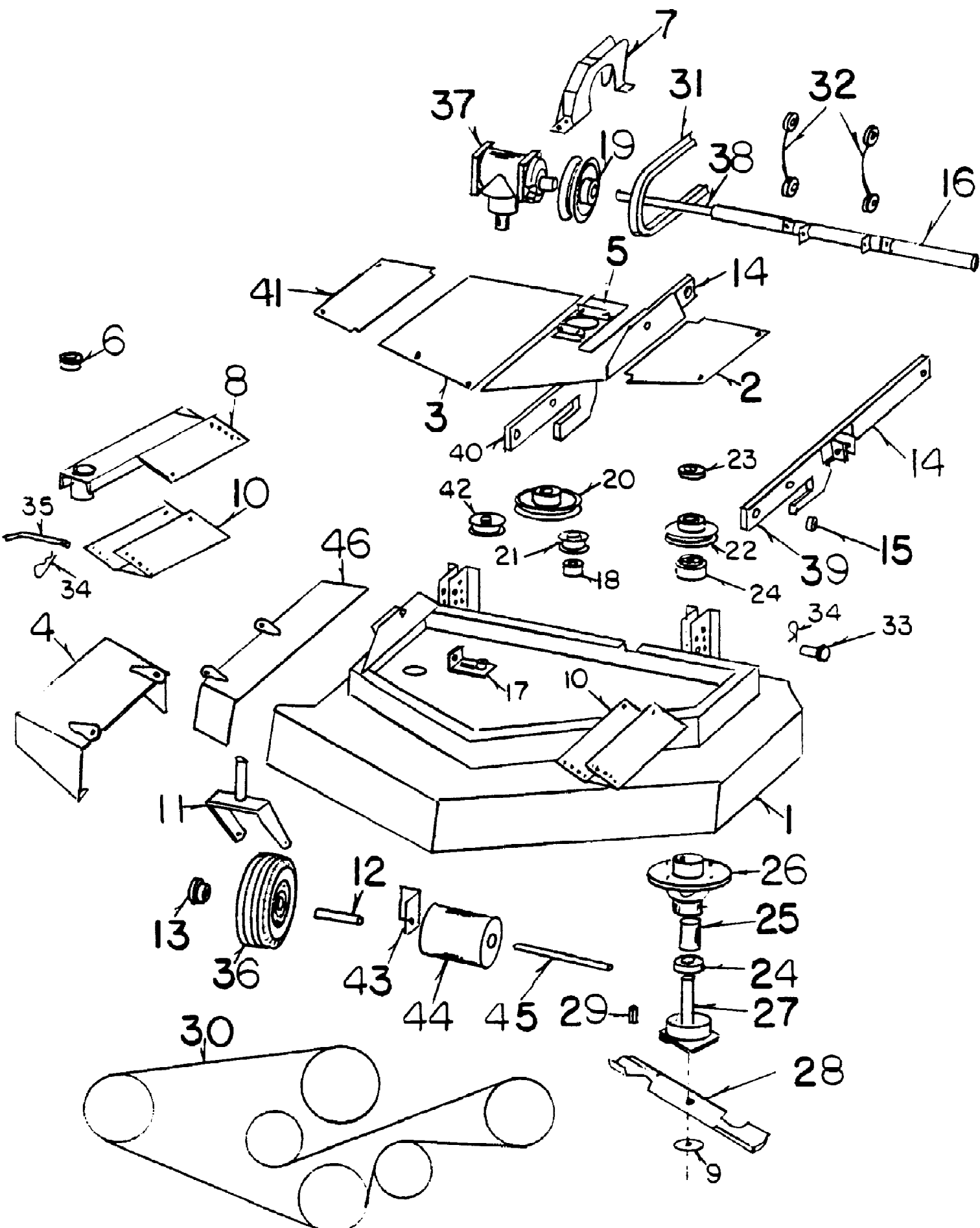
Belt Placement Diagram
