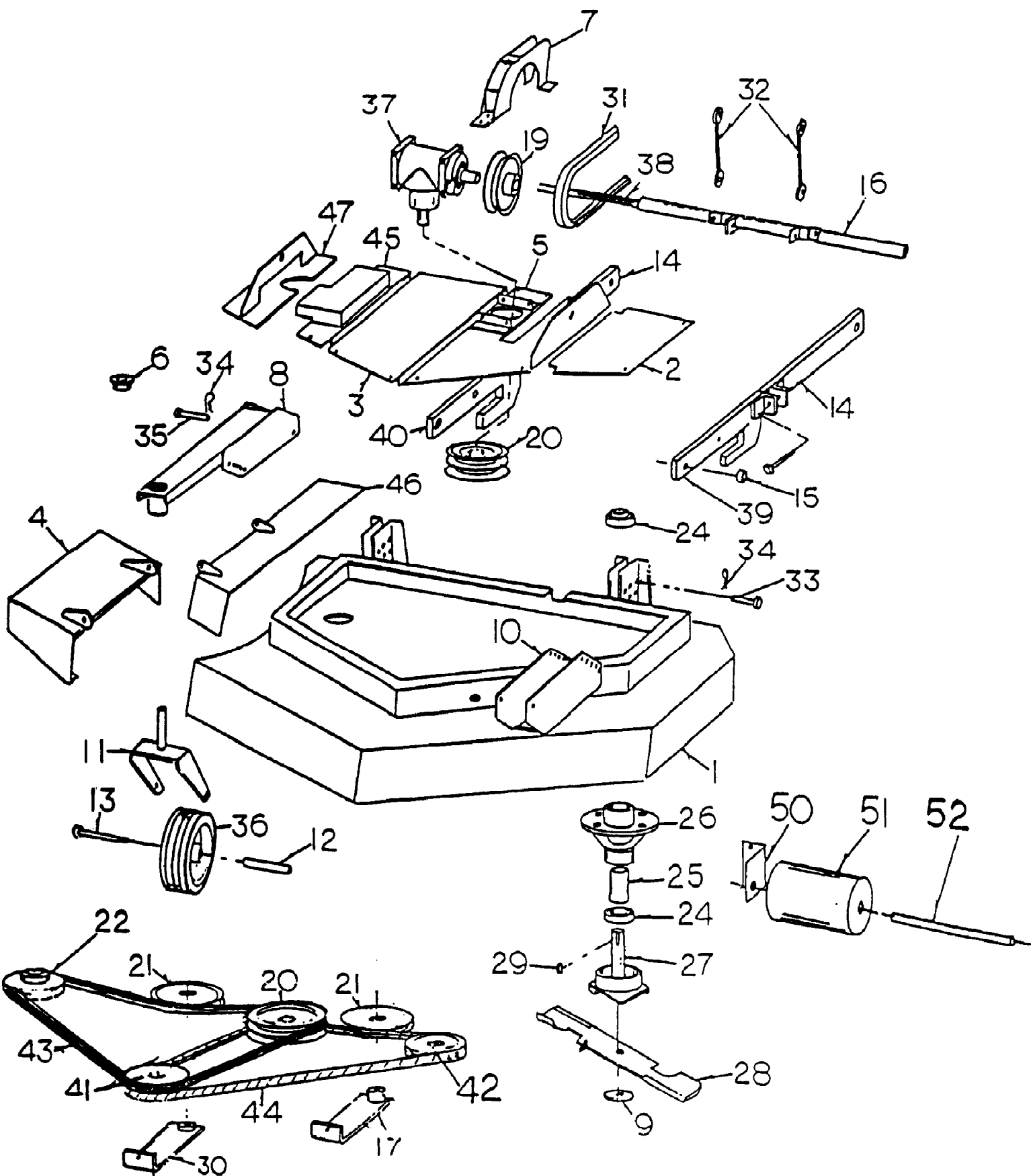
Belt Placement Diagram
